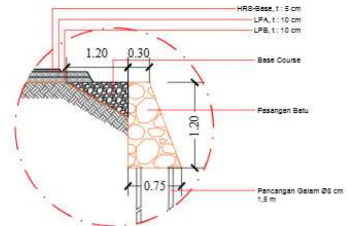
DETAIL POTONGAN
