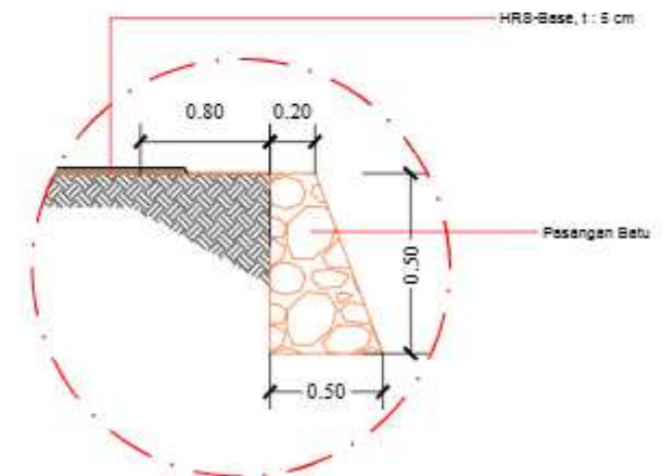
DETAIL POTONGAN
