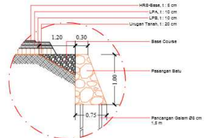
DETAIL POTONGAN
