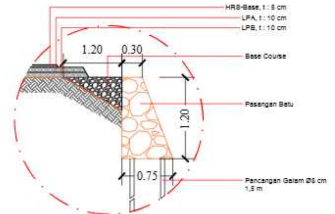
DETAIL POTONGAN
