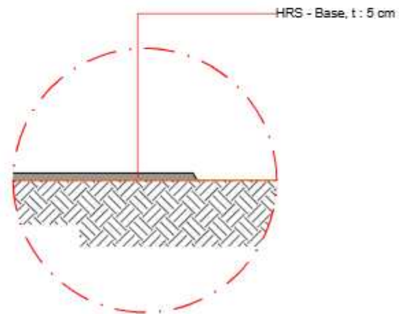
DETAIL POTONGAN
