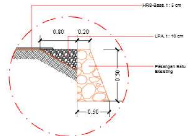
DETAIL POTONGAN
