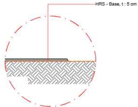
DETAIL POTONGAN
