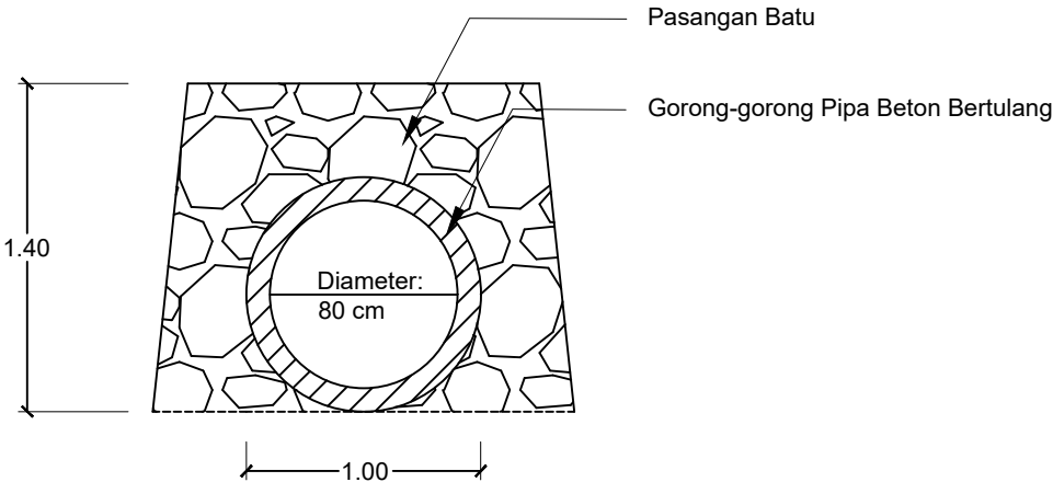
Detail Rencana Gorong-Gorong Skala 1 : 25
